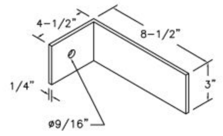
BRACKET DETAIL
