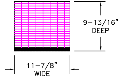
TREAD PLAN VIEW (TREADS ARE 11" DEEP FOR 56° AT)
