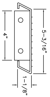
B ALUMINUM TREAD (6005-T5)
