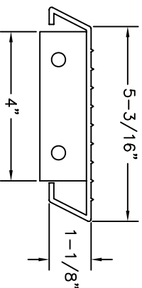
(B) ALUMINUM TREAD (6005-T5)
