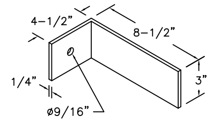
BRACKET DETAIL
